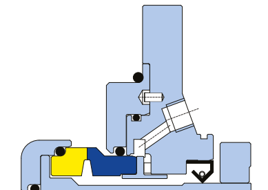
FGDSS-NL™ — Australian backplate
